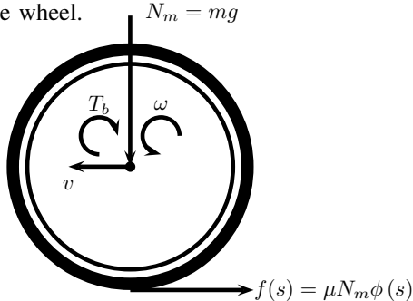
Fig. 2. Wheel forces and torques
