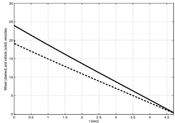
Fig. 6. Wheel velocity x_1 (dashed) and vehicle velocity x_3 (solid)
