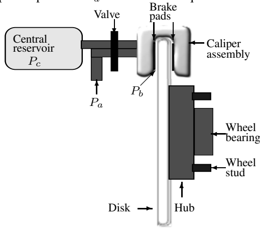
Fig. 1. Pneumatic brake scheme
