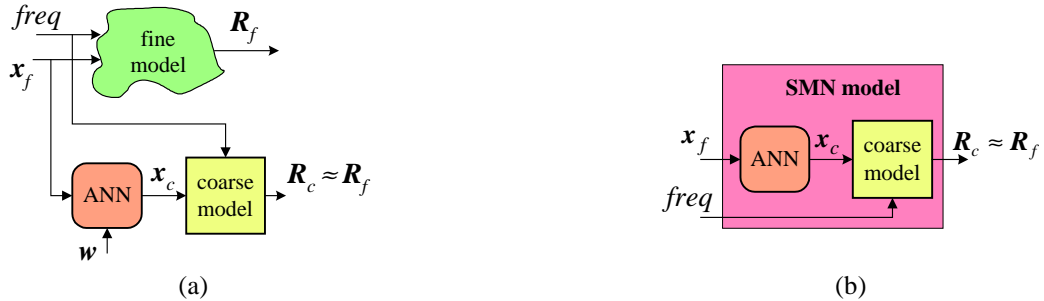
Fig. 2. Space-Mapped Neuromodeling concept: (a) SM neuromodeling, (b) SMN model.
