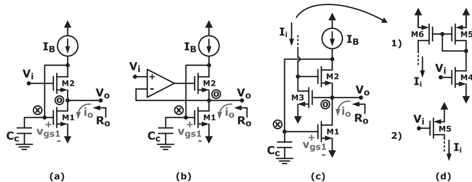
Fig. 1. a) Conventional Flipped Voltage Follower (FVF) [1], b) FVF with input op-amp to enhance the output resistance [5, 6], c) Proposed FVF circuit including a regulated cascode stage, and d) examples of transconductors to provide the input current I_i from an input voltage V_i .
