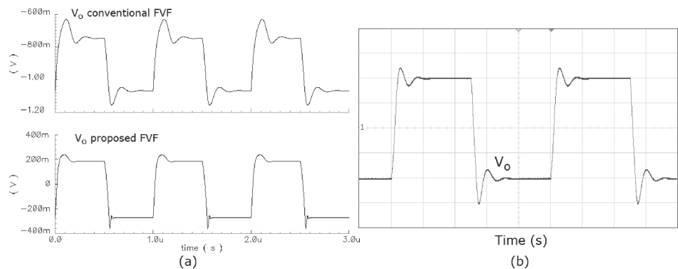
Fig. 4. a) Simulated transient response of the conventional FVF in [1] and the proposed circuit for a square input signal of V_i = 0.4 V_{\text{pp}} at 1 MHz driving a loading capacitor of C_L = 15\text{ pF} ; and b) experimental response of the proposed circuit for an input signal of V_i = 0.4 V_{\text{pp}} at 100 kHz with C_L = 55\text{ pF} (x axes is 2\ \mu\text{sec}/\square , and y axes is 100\ \text{mV}/\square ).
