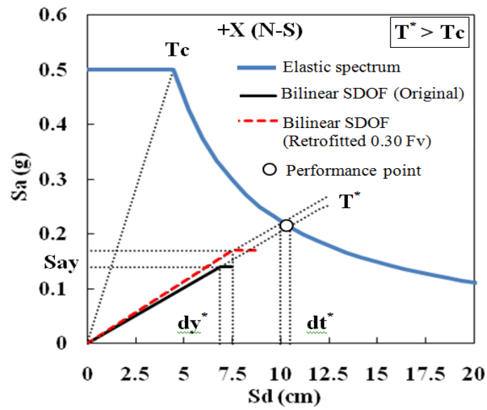
Figure 9: Seismic evaluation of the north bell tower of the Cathedral of Colima by the Capacity Spectrum method: (a) -X direction and (b) +X direction (springs)
