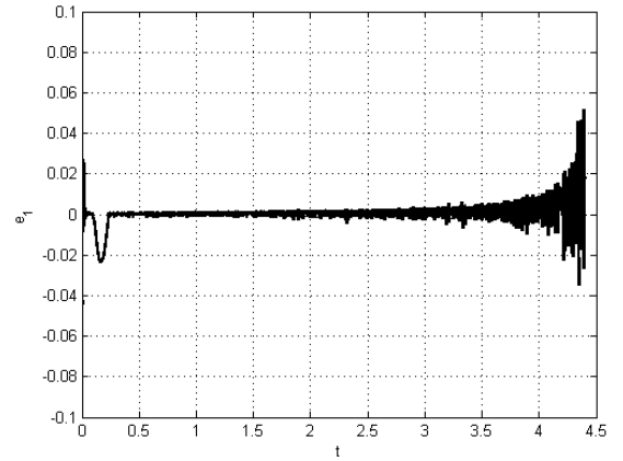
Fig. 7. Tracking error, e_1 = y - y_{ref}
