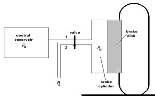
Fig. 1. Pneumatic brake model
