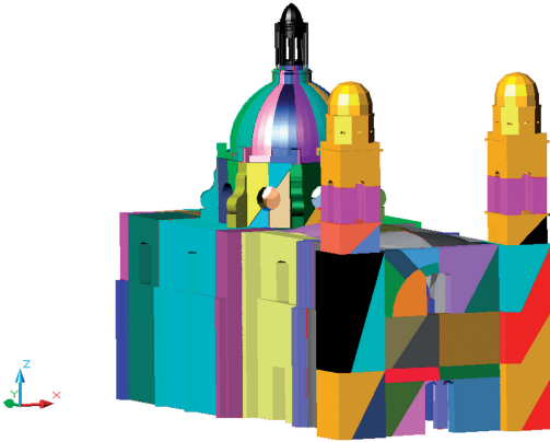
Figure 7. Full model of the cathedral.
